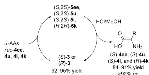
Scheme 1. Disassembly of diastereomerically pure (S,2S)-5ee, (S,2S)-5u, (S,2S)-5l, and (R,2R)-5k, and isolation of the free target \alpha -AAs (S)-4ee, (S)-4u, (S)-4l, and (R)-4k along with the recycling and reuse of the chiral ligands (S)-3 and (R)-3.
