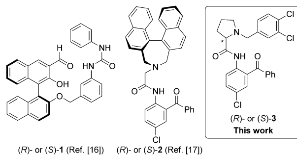
Figure 1. The previously reported ligands 1 and 2 , which contain axially chiral 1,1'-binaphthyl moieties, and the structurally advantageous proline-derived ligands 3 , which were used in this work.
